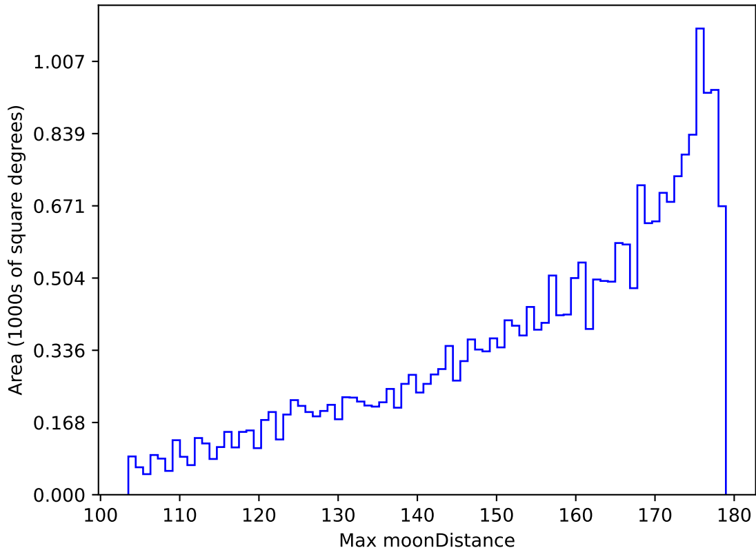
weather_cloudso31v3.4_10yrs All sky g band: Max moonDistance
