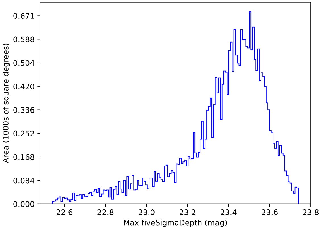
weather_cloudso31v3.4_10yrs Yr 1 z band: Max fiveSigmaDepth
