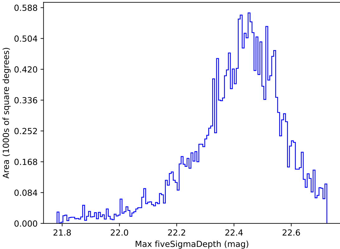
weather_cloudso31v3.4_10yrs Yr 1 y band: Max fiveSigmaDepth
