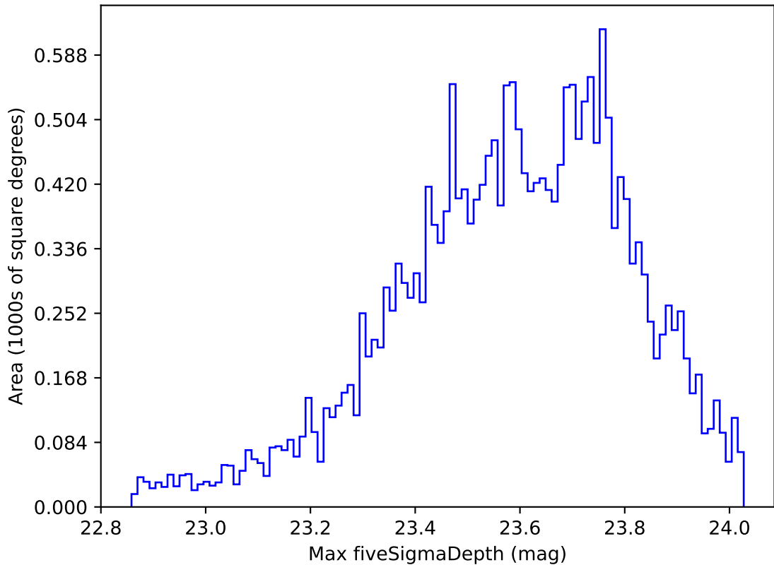
weather_cloudso31v3.4_10yrs Yr 1 u band: Max fiveSigmaDepth
