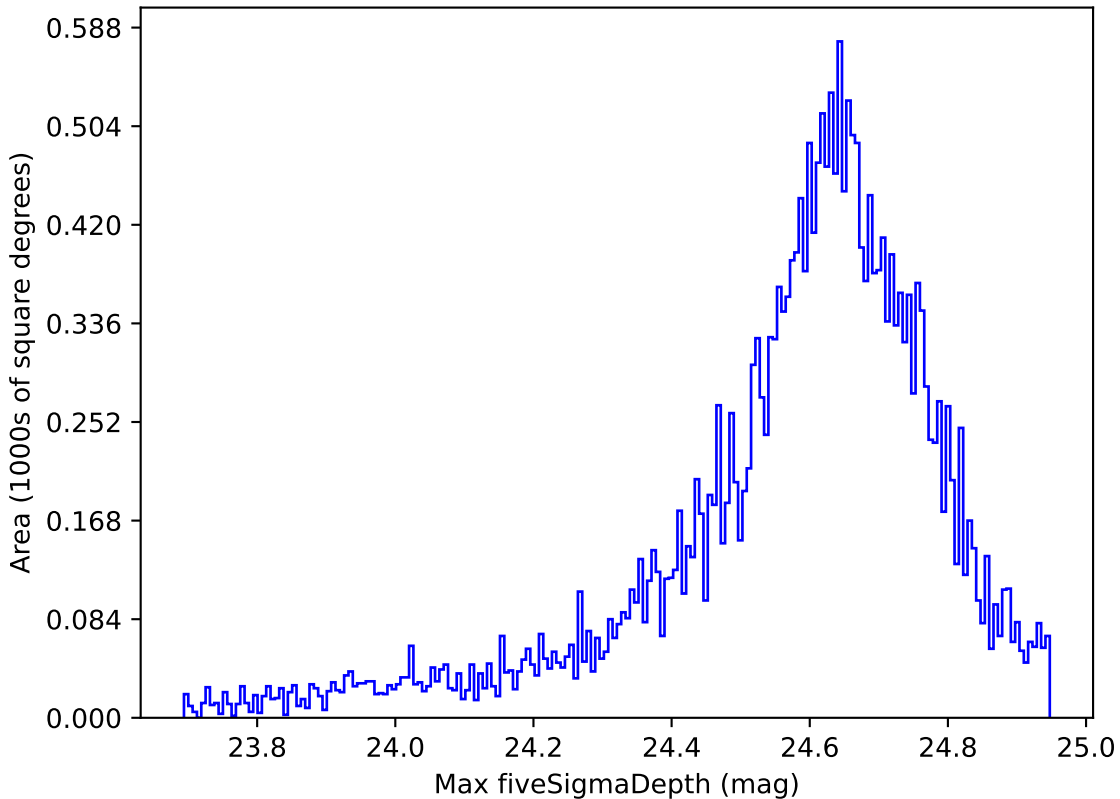
weather_cloudso31v3.4_10yrs Yr 1 r band: Max fiveSigmaDepth
