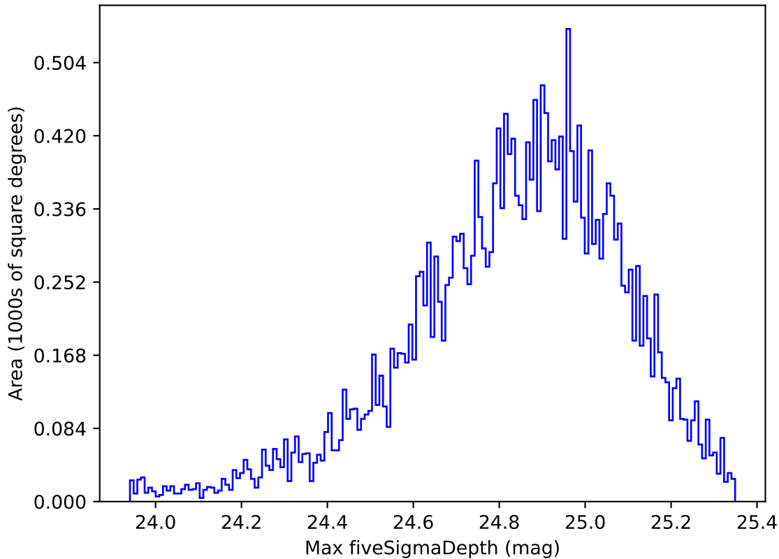
weather_cloudso31v3.4_10yrs Yr 1 g band: Max fiveSigmaDepth
