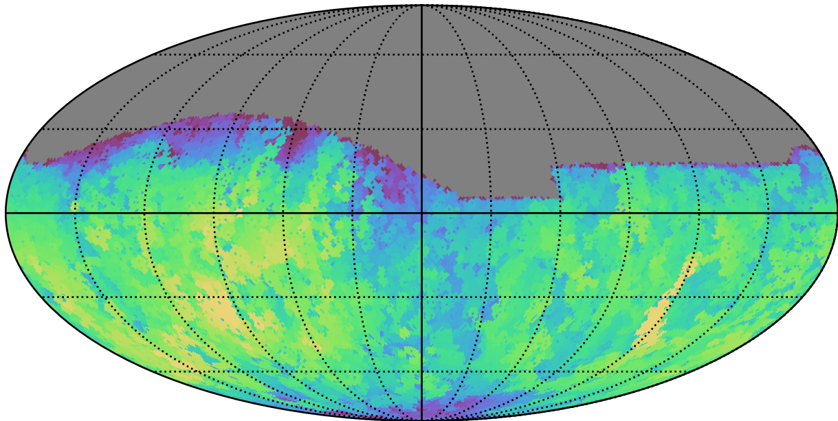
weather_cloudso31v3.4_10yrs Yr 1 all bands: Max fiveSigmaDepth
