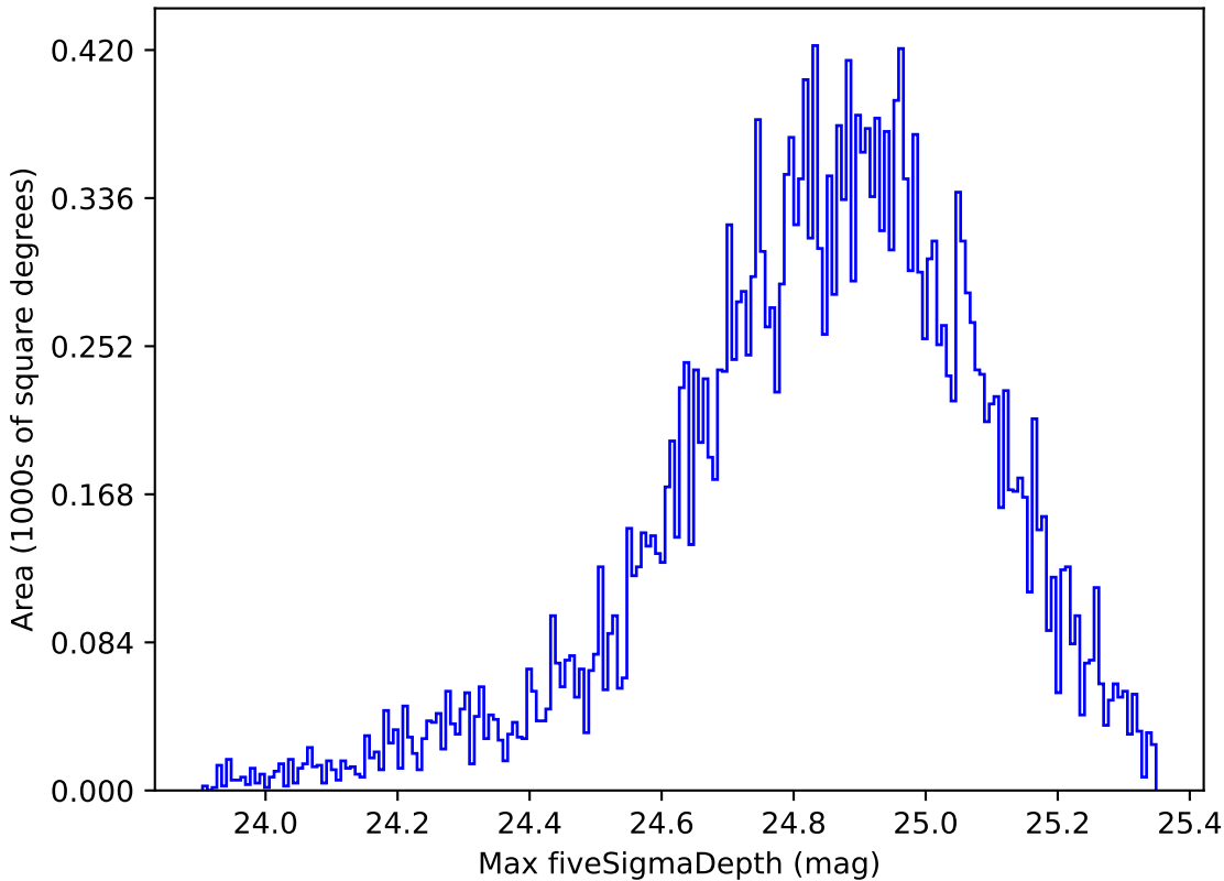
weather_cloudso31v3.4_10yrs Yr 1 all bands: Max fiveSigmaDepth
