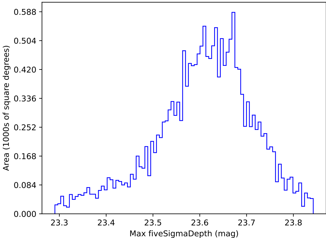
weather_cloudso31v3.4_10yrs WFD z band: Max fiveSigmaDepth
