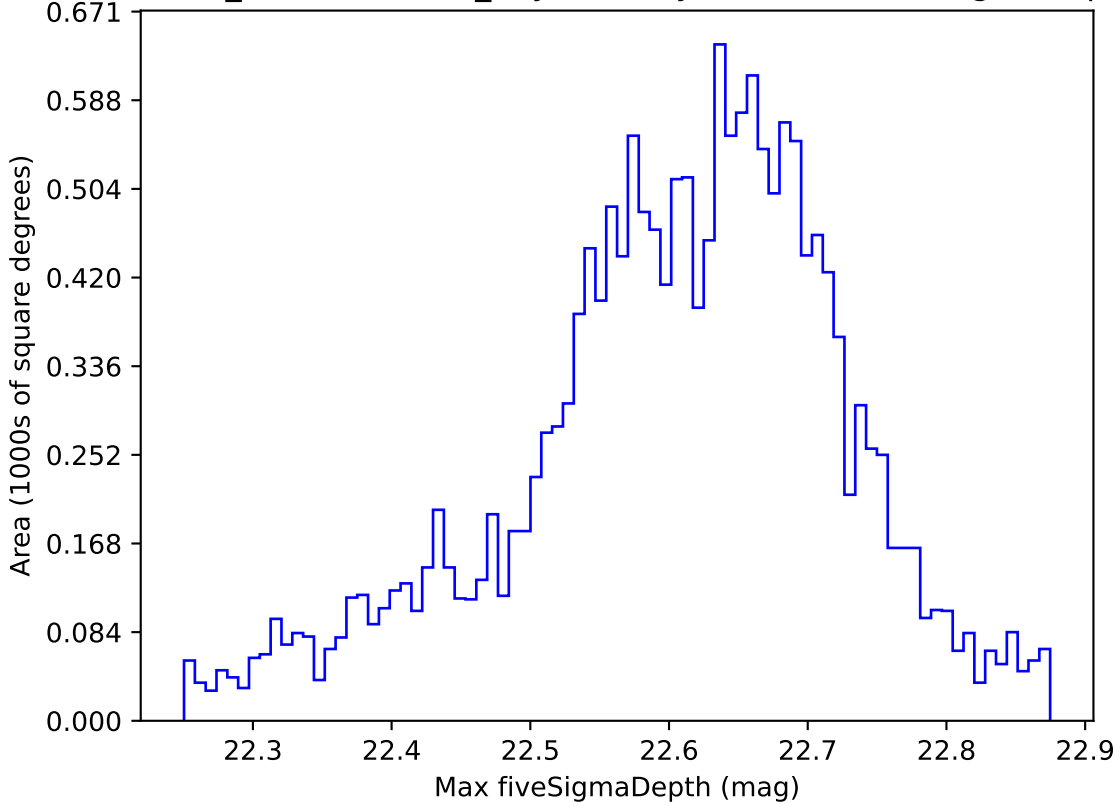
weather_cloudso31v3.4_10yrs WFD y band: Max fiveSigmaDepth
