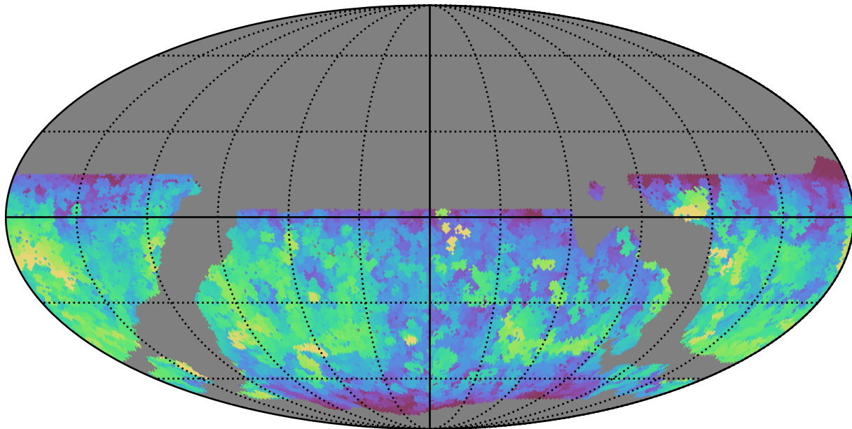
weather_cloudso31v3.4_10yrs WFD u band: Max fiveSigmaDepth
