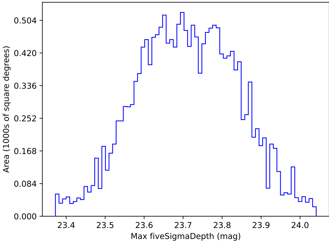
weather_cloudso31v3.4_10yrs WFD u band: Max fiveSigmaDepth
