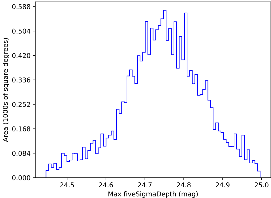
weather_cloudso31v3.4_10yrs WFD r band: Max fiveSigmaDepth
