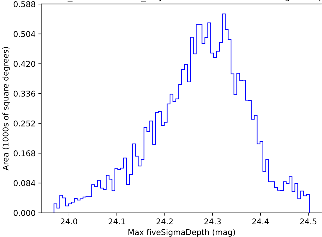
weather_cloudso31v3.4_10yrs WFD i band: Max fiveSigmaDepth
