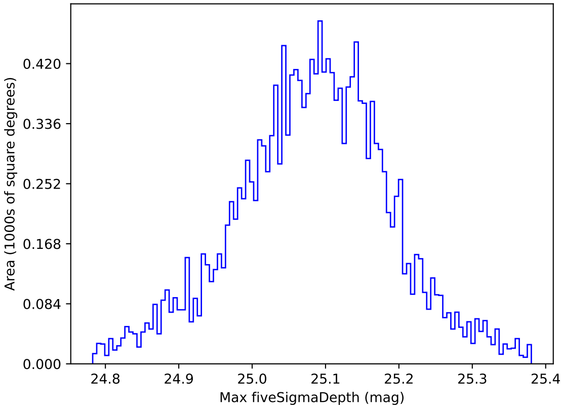
weather_cloudso31v3.4_10yrs WFD g band: Max fiveSigmaDepth
