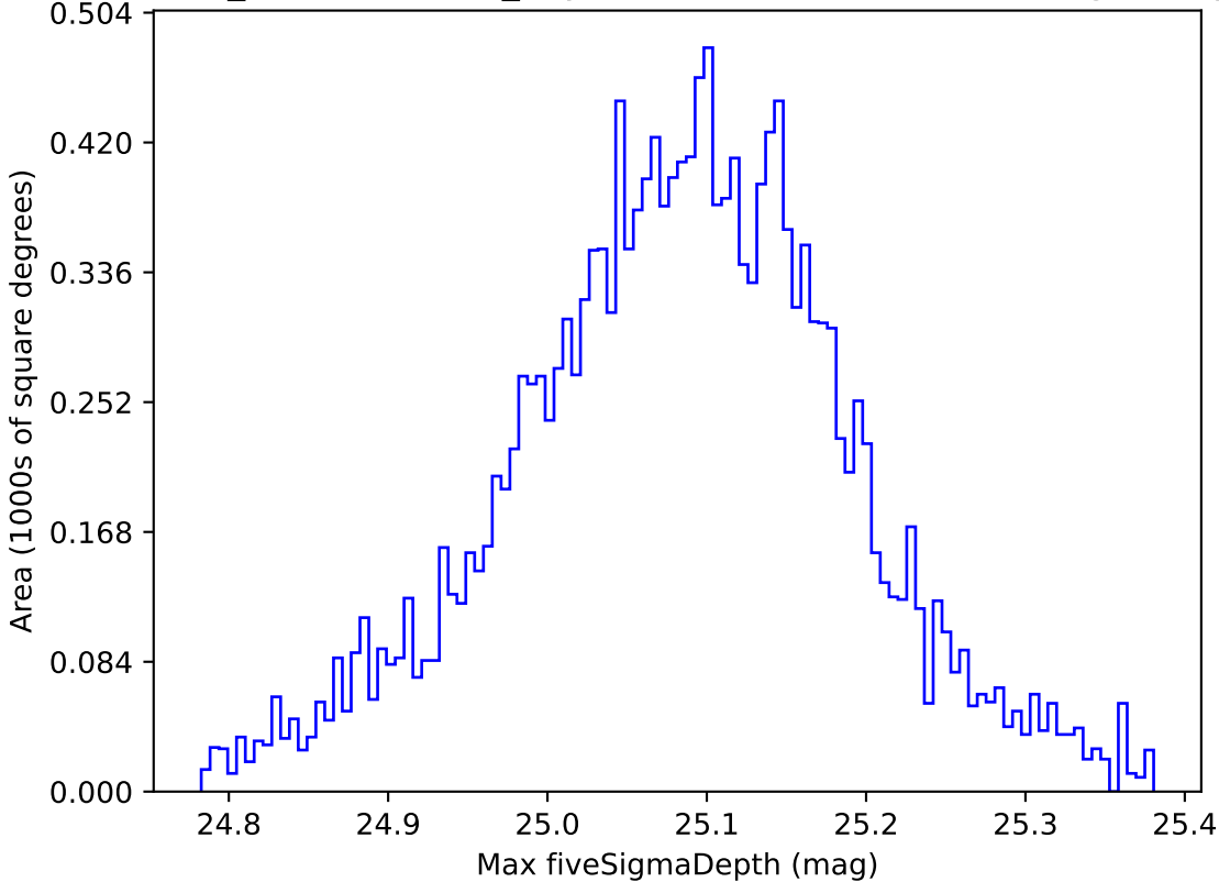
weather_cloudso31v3.4_10yrs WFD all bands: Max fiveSigmaDepth
