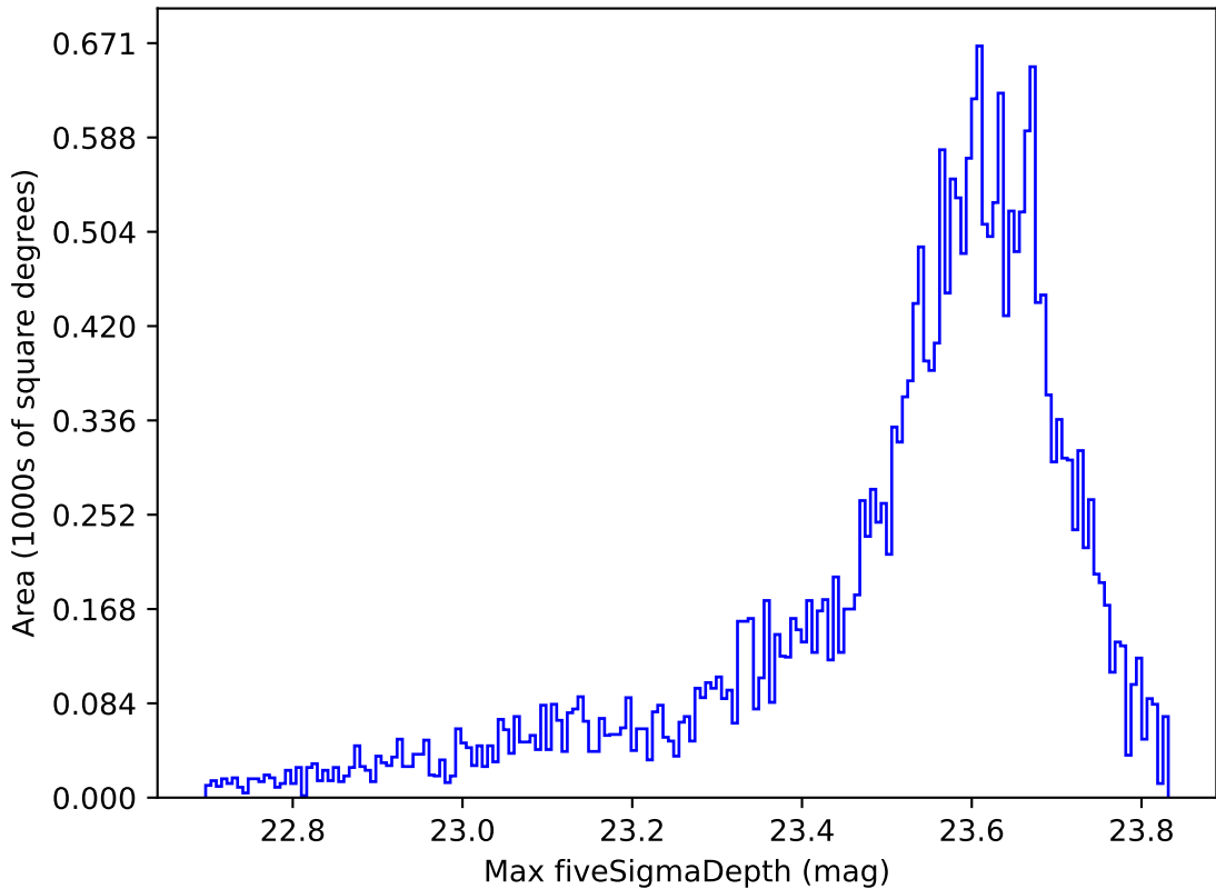
weather_cloudso31v3.4_10yrs All sky z band: Max fiveSigmaDepth
