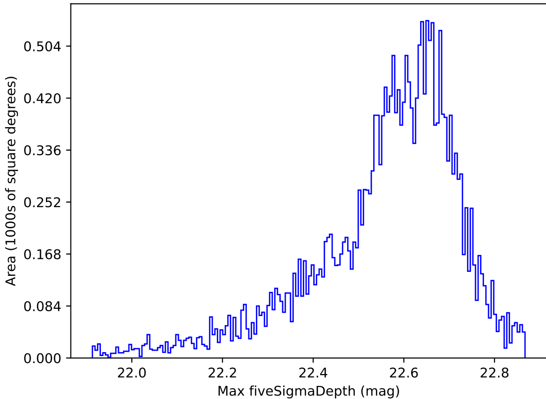
weather_cloudso31v3.4_10yrs All sky y band: Max fiveSigmaDepth
