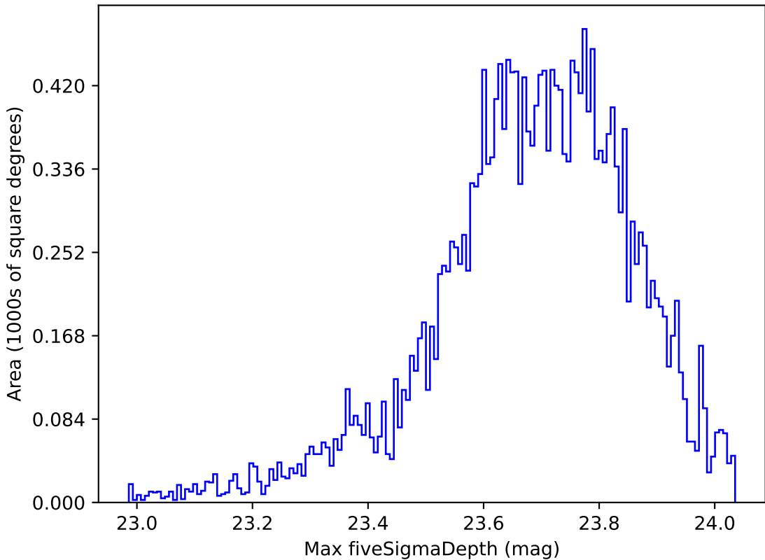
weather_cloudso31v3.4_10yrs All sky u band: Max fiveSigmaDepth
