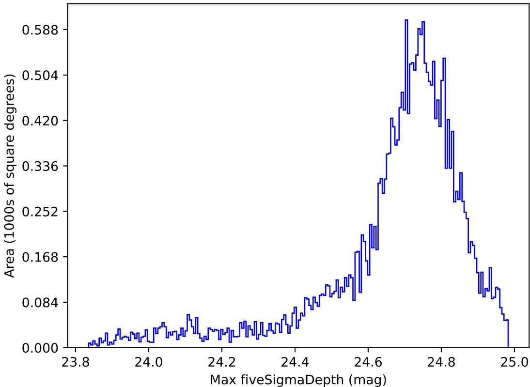
weather_cloudso31v3.4_10yrs All sky r band: Max fiveSigmaDepth
