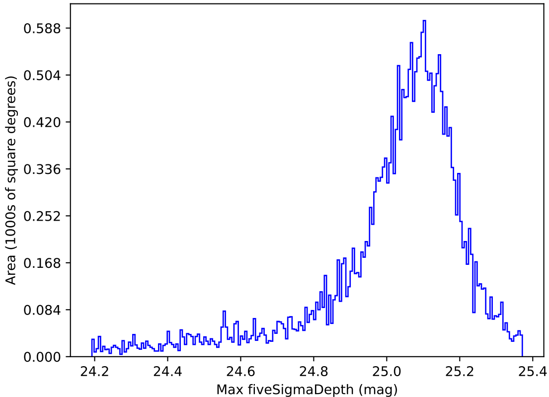
weather_cloudso31v3.4_10yrs All sky g band: Max fiveSigmaDepth
