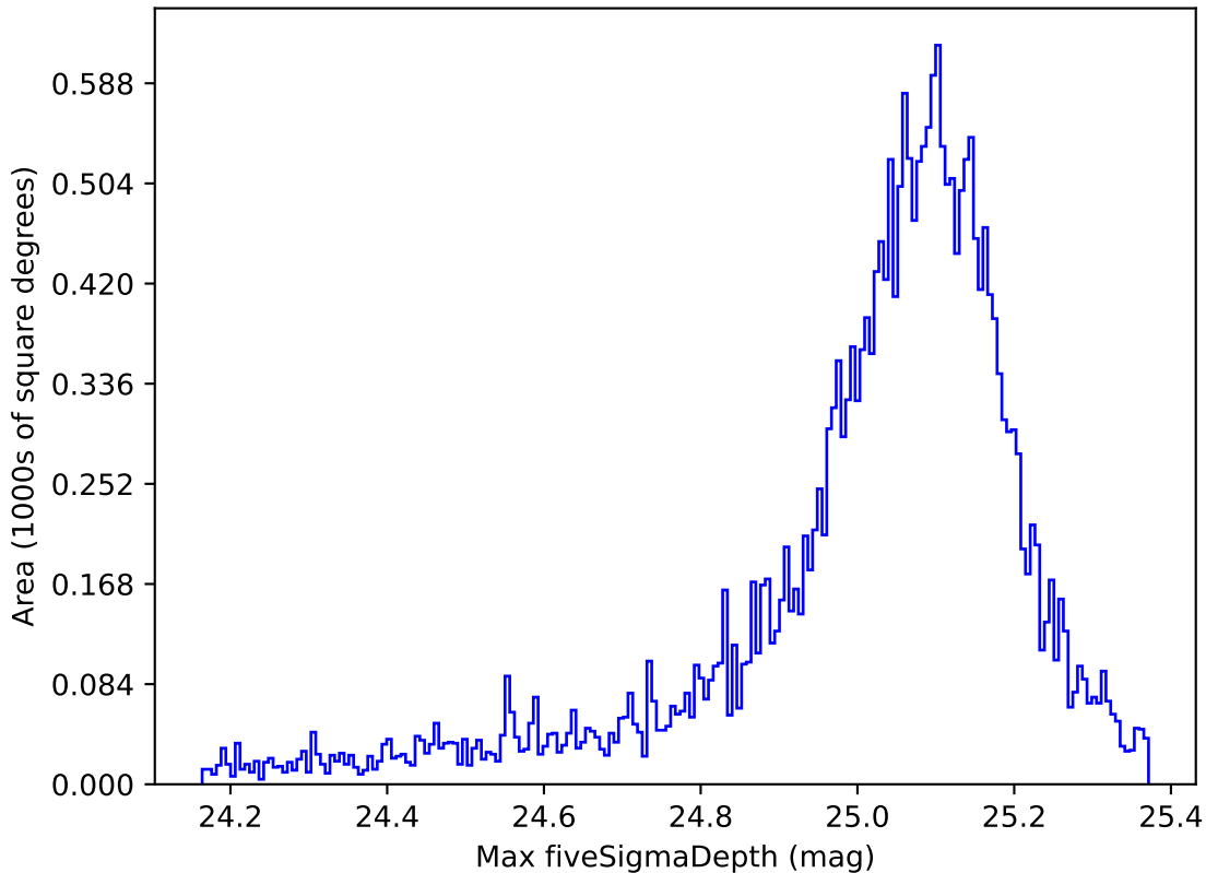
weather_cloudso31v3.4_10yrs All sky all bands: Max fiveSigmaDepth
