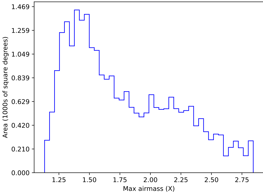
weather_cloudso31v3.4_10yrs Yr 1 z band: Max airmass
