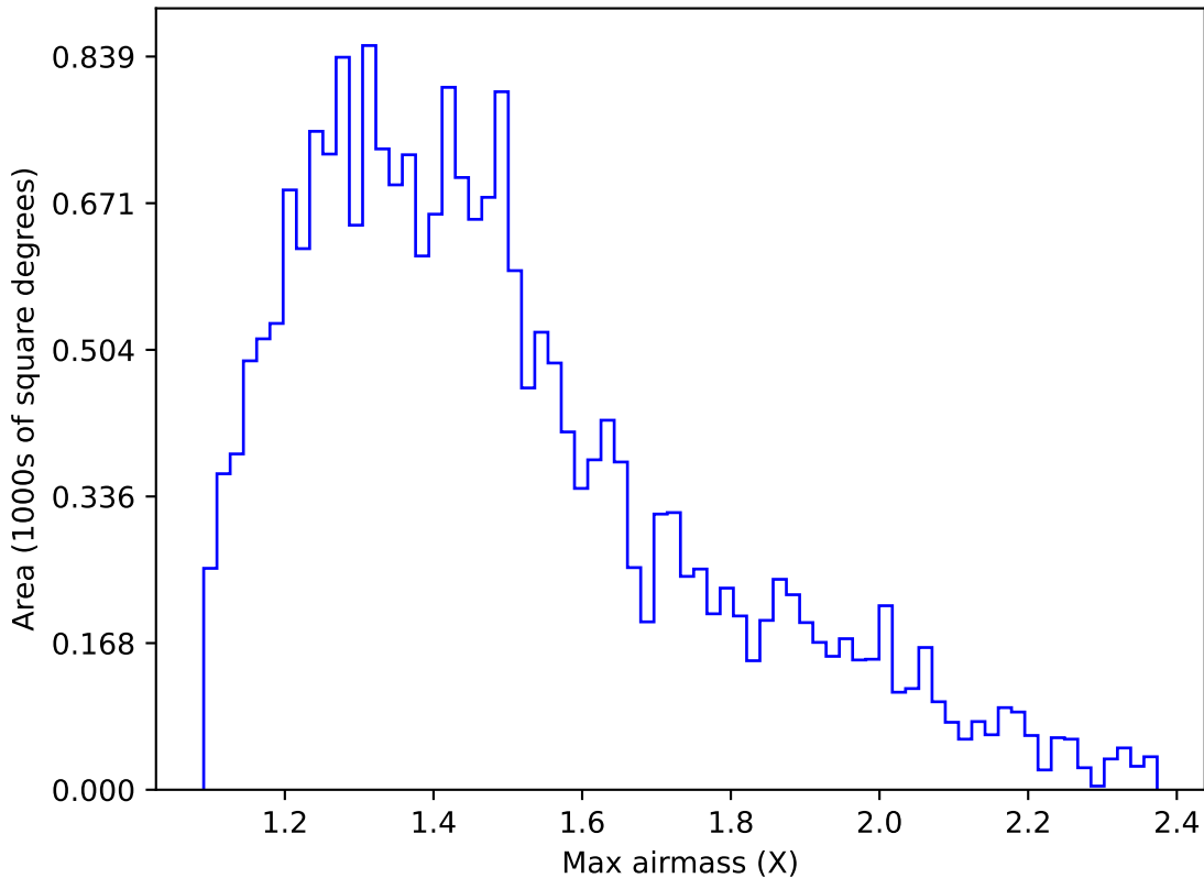
weather_cloudso31v3.4_10yrs Yr 1 u band: Max airmass
