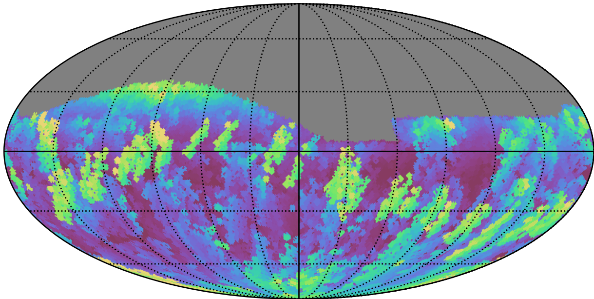
weather_cloudso31v3.4_10yrs Yr 1 r band: Max airmass
