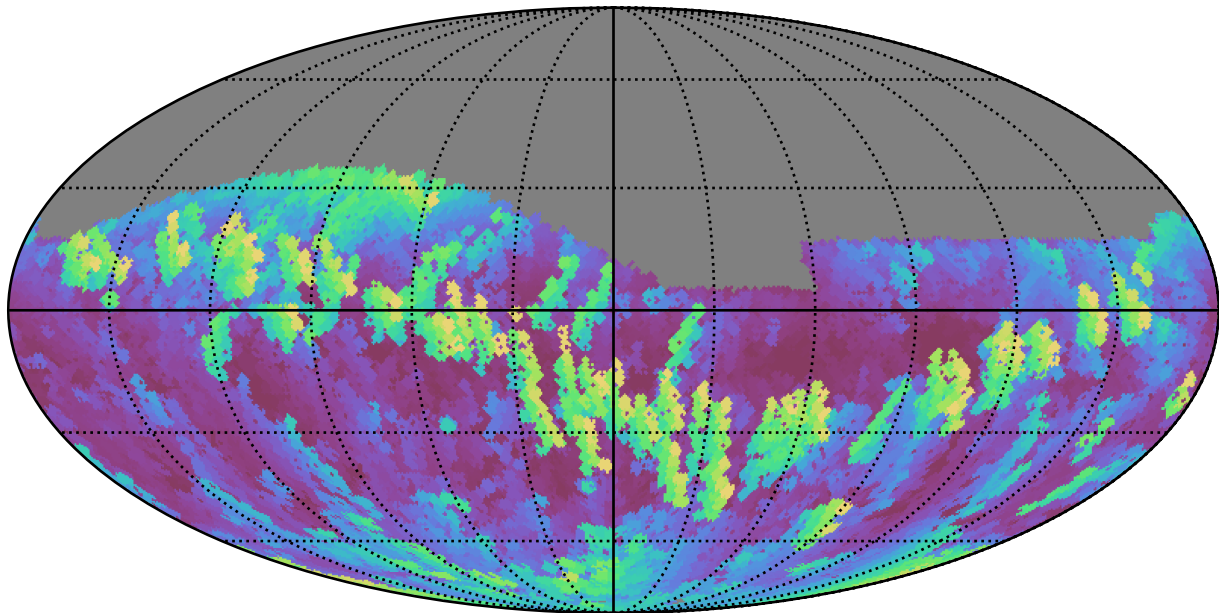
weather_cloudso31v3.4_10yrs Yr 1 i band: Max airmass
