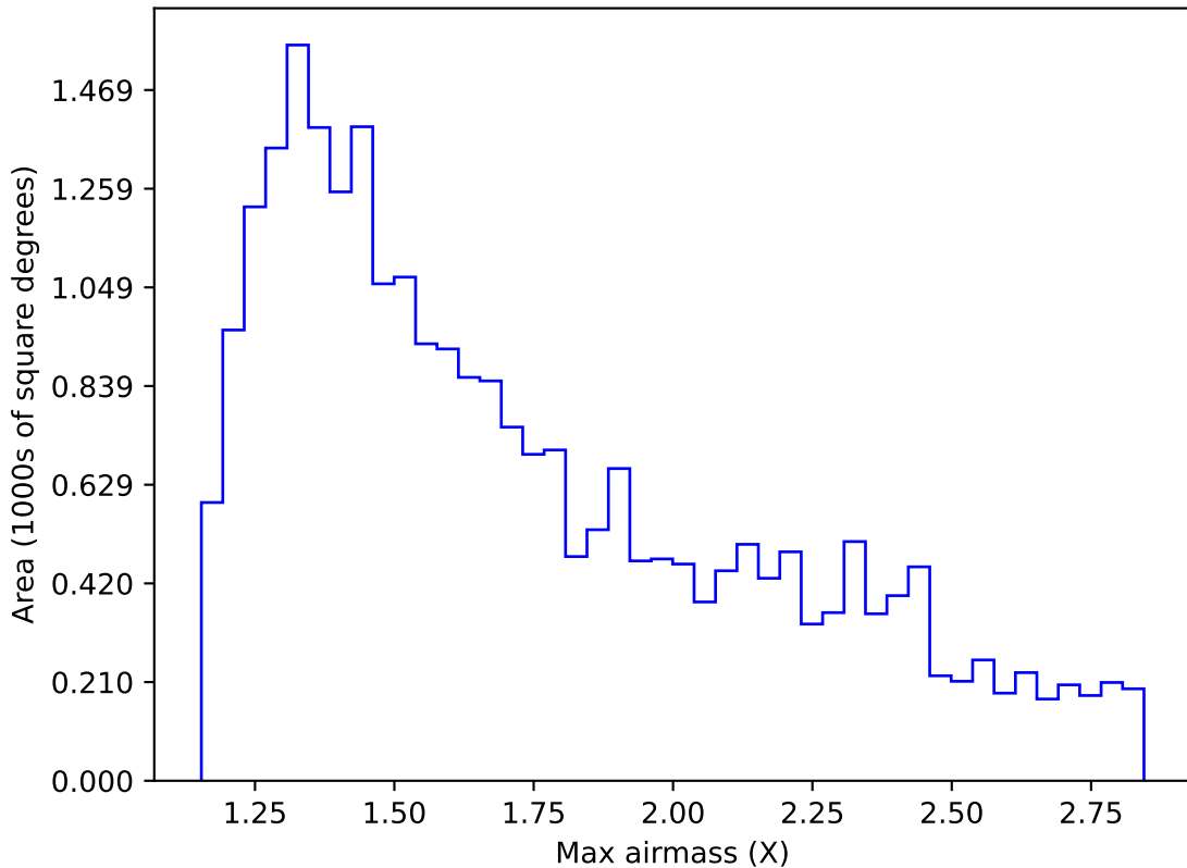
weather_cloudso31v3.4_10yrs Yr 1 i band: Max airmass
