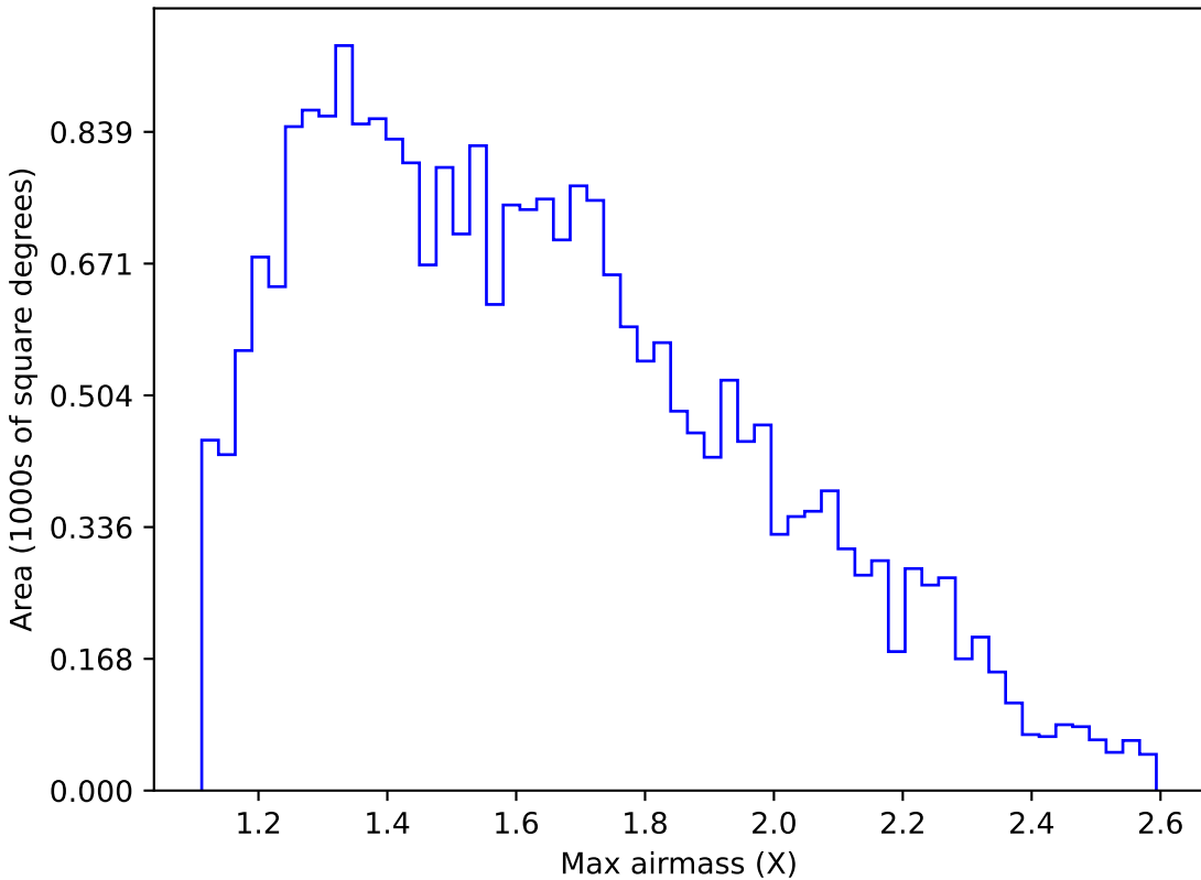
weather_cloudso31v3.4_10yrs Yr 1 g band: Max airmass
