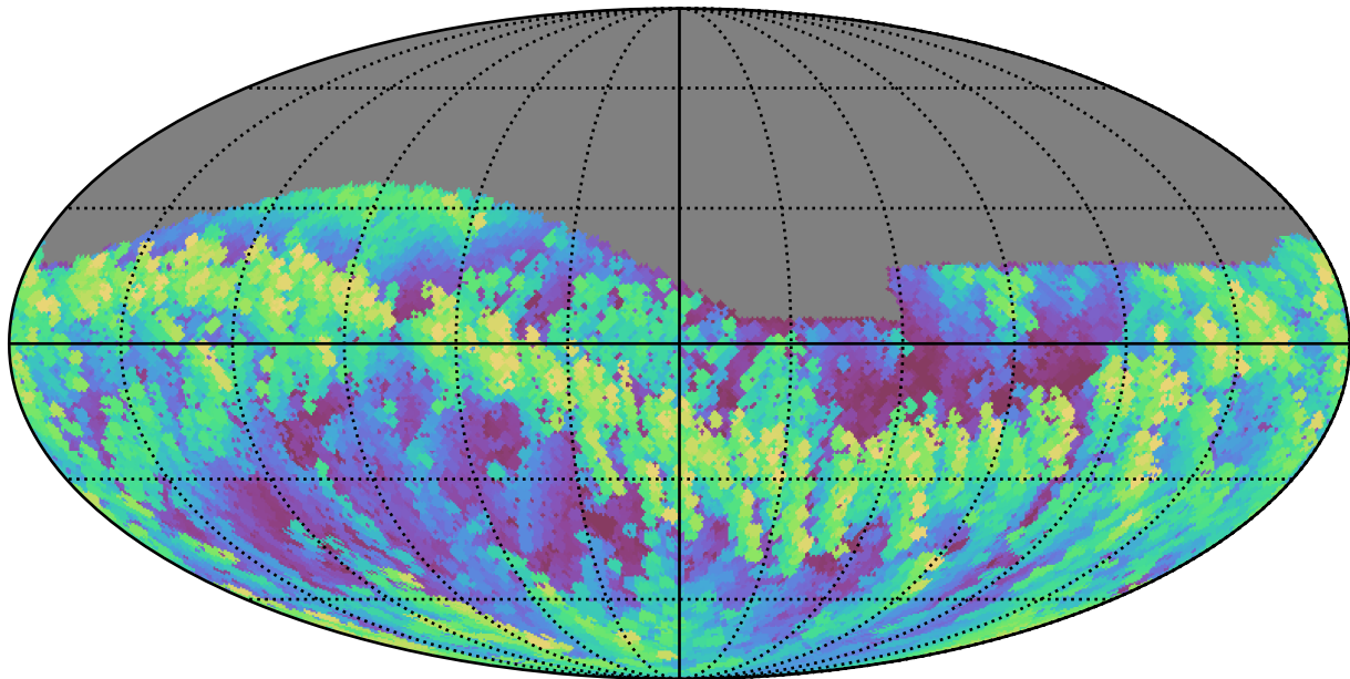
weather_cloudso31v3.4_10yrs Yr 1 all bands: Max airmass
