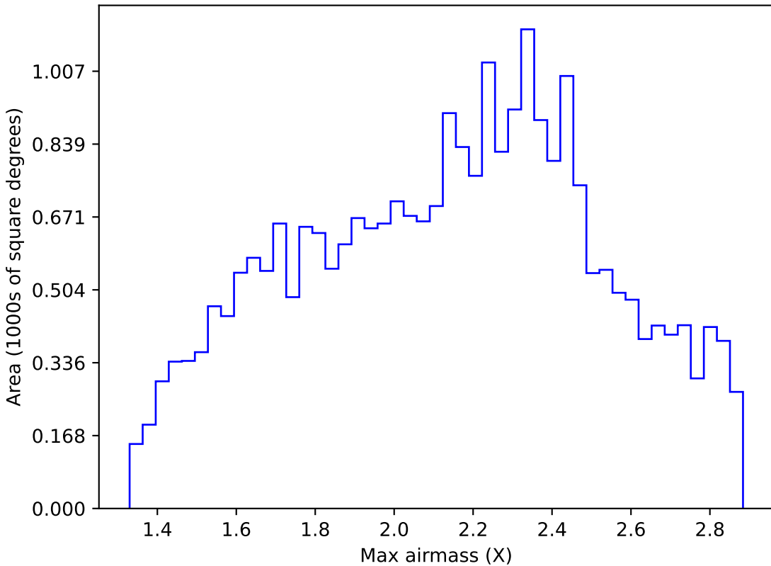
weather_cloudso31v3.4_10yrs Yr 1 all bands: Max airmass
