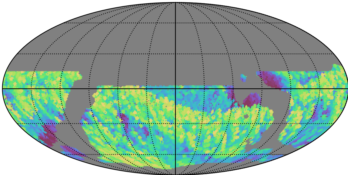
weather_cloudso31v3.4_10yrs WFD z band: Max airmass
