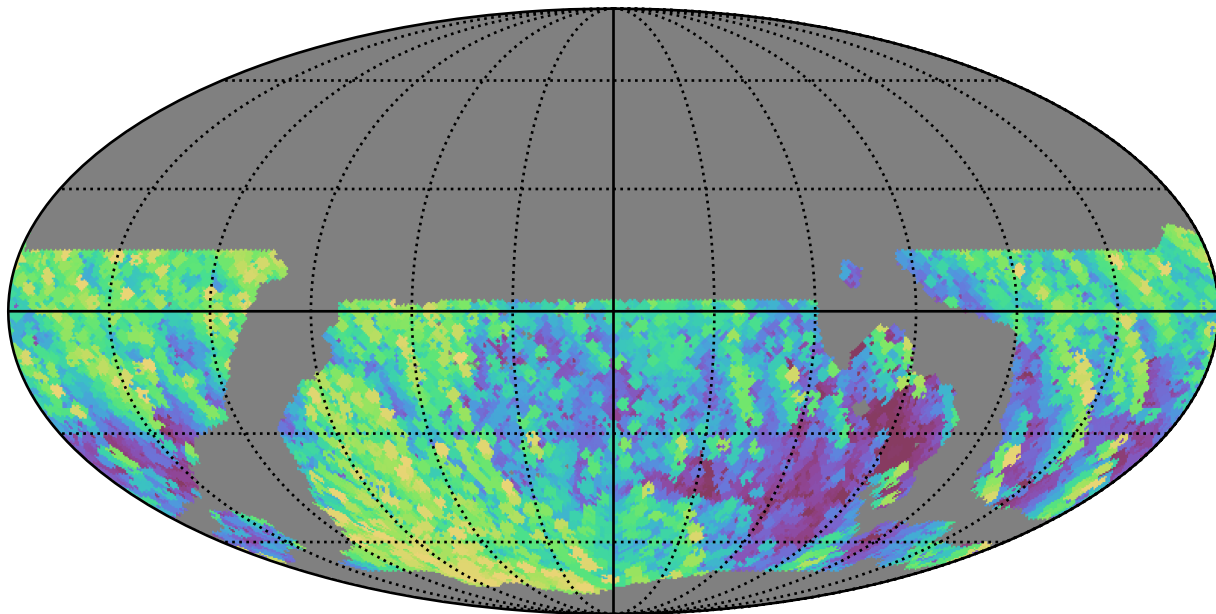
weather_cloudso31v3.4_10yrs WFD y band: Max airmass
