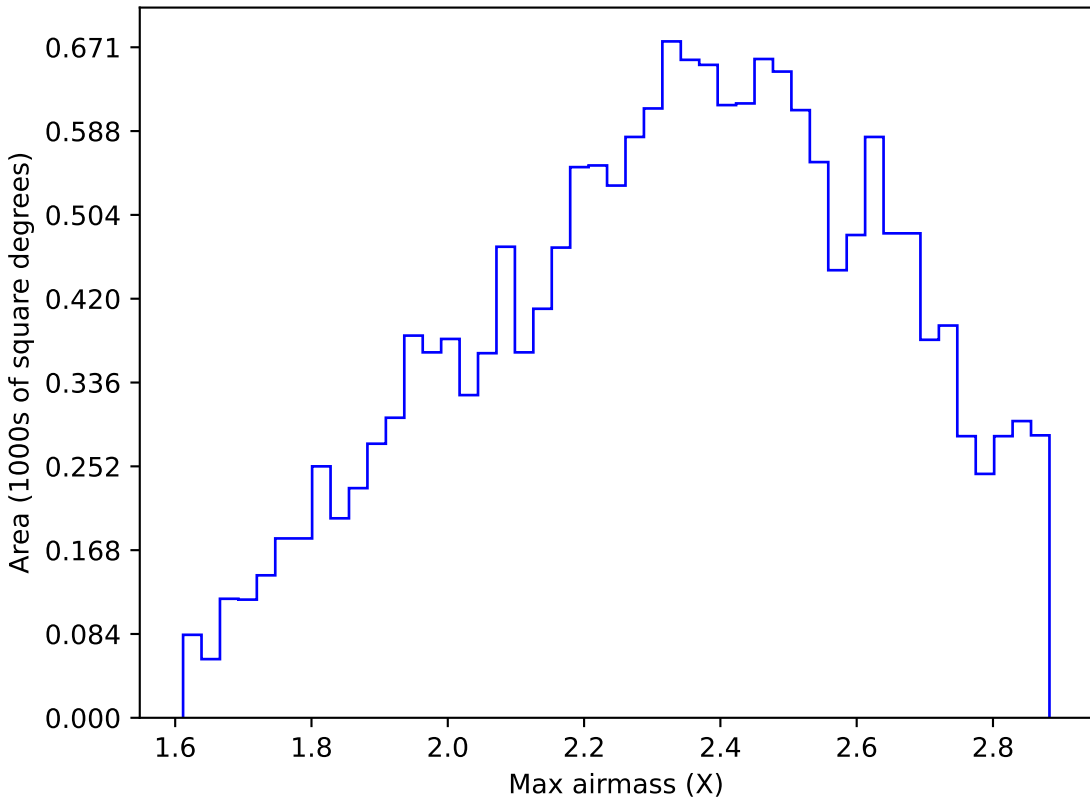
weather_cloudso31v3.4_10yrs WFD y band: Max airmass
