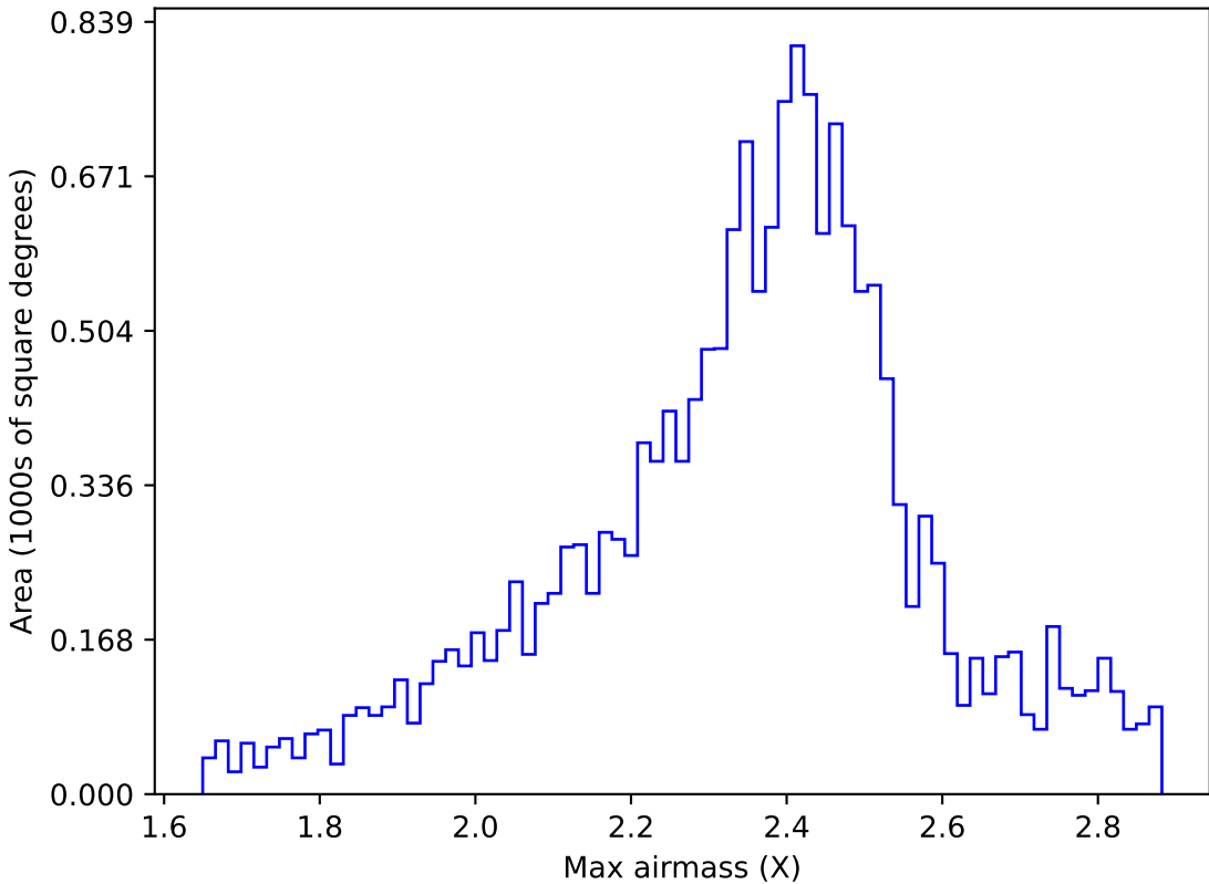
weather_cloudso31v3.4_10yrs WFD r band: Max airmass
