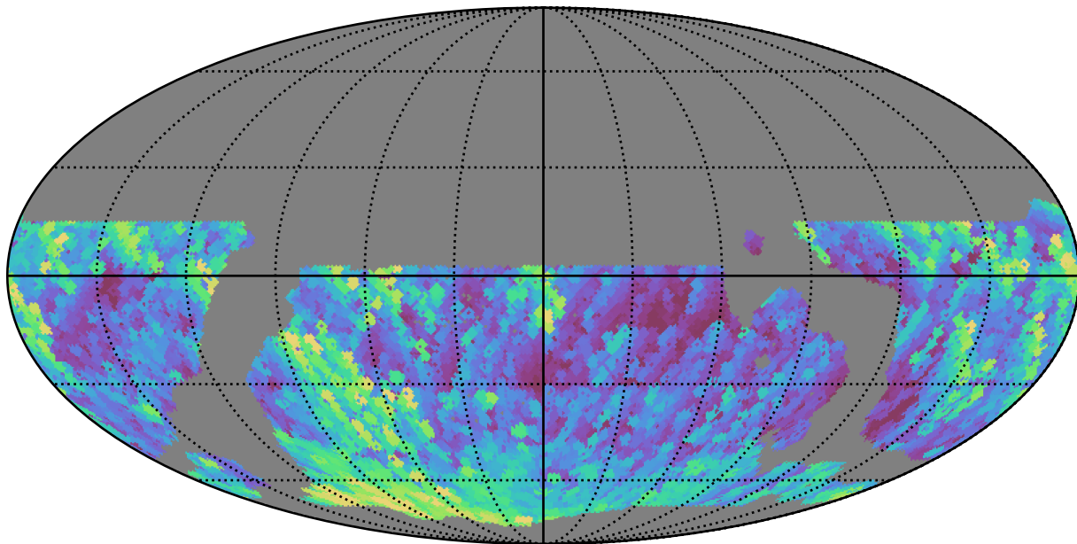
weather_cloudso31v3.4_10yrs WFD g band: Max airmass
