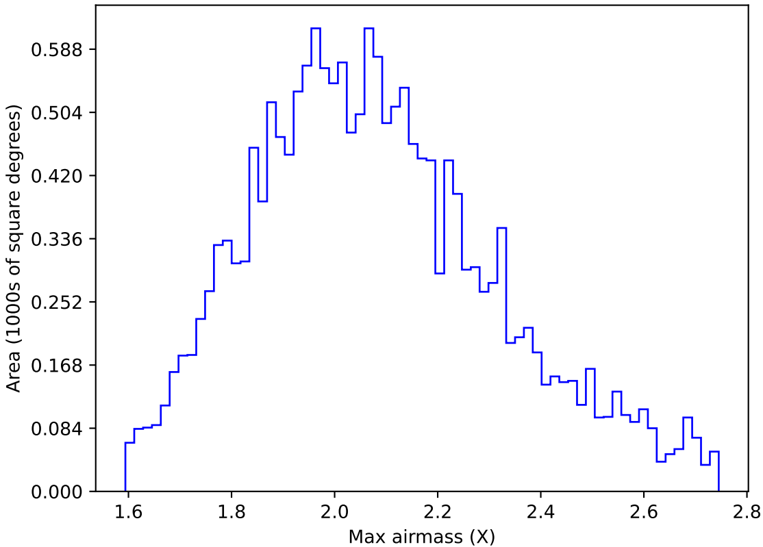
weather_cloudso31v3.4_10yrs WFD g band: Max airmass
