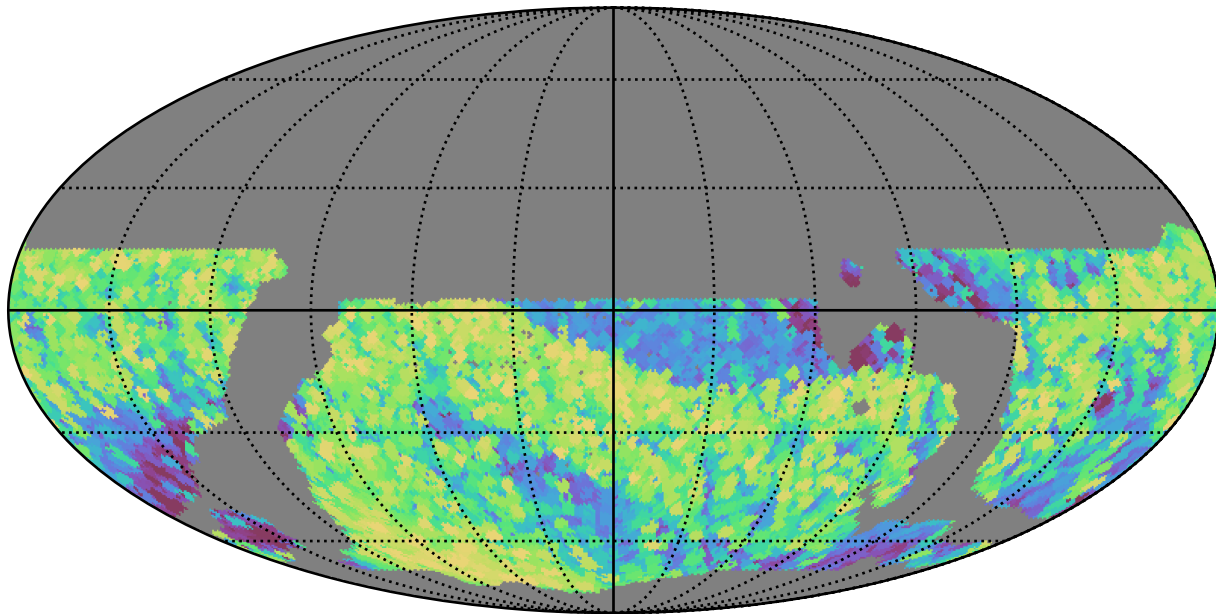
weather_cloudso31v3.4_10yrs WFD all bands: Max airmass
