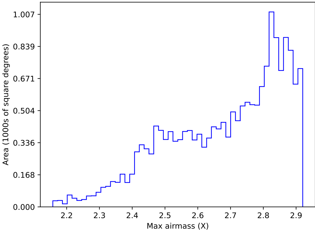
weather_cloudso31v3.4_10yrs WFD all bands: Max airmass
