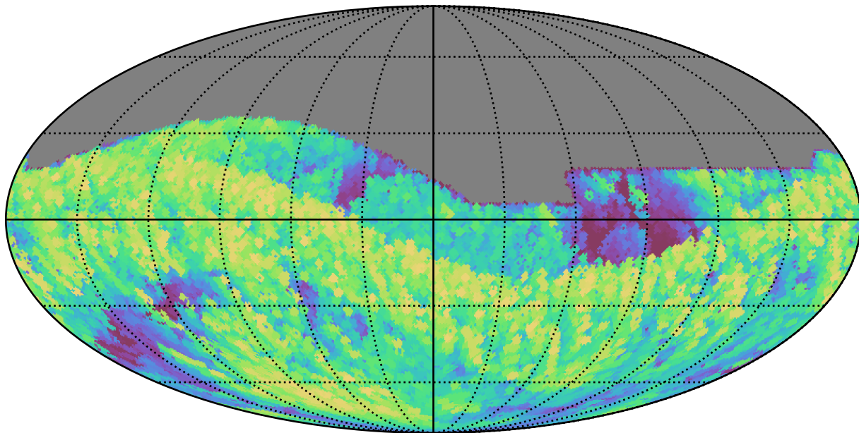
weather_cloudso31v3.4_10yrs All sky z band: Max airmass
