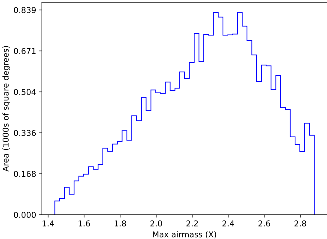
weather_cloudso31v3.4_10yrs All sky y band: Max airmass
