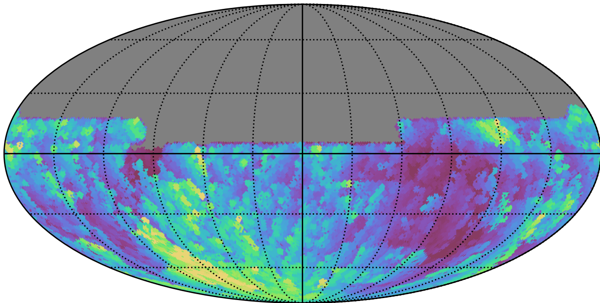
weather_cloudso31v3.4_10yrs All sky u band: Max airmass
