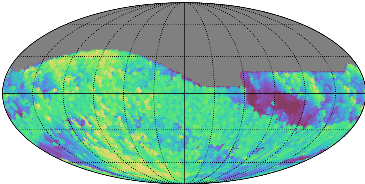
weather_cloudso31v3.4_10yrs All sky r band: Max airmass
