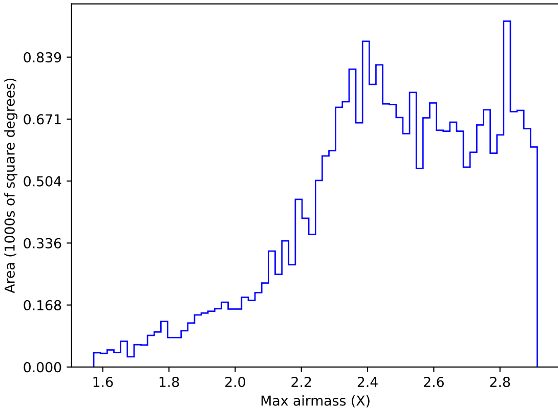
weather_cloudso31v3.4_10yrs All sky i band: Max airmass
