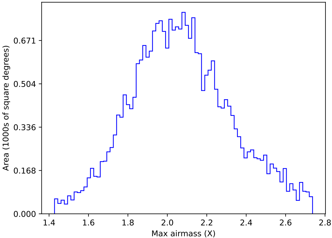
weather_cloudso31v3.4_10yrs All sky g band: Max airmass
