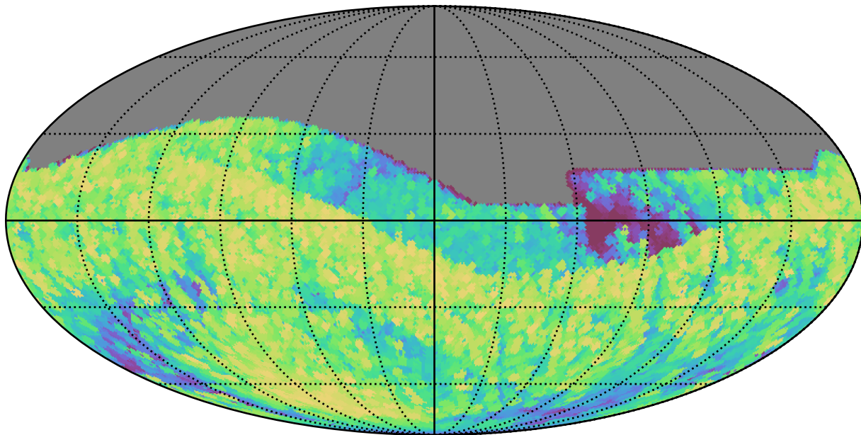
weather_cloudso31v3.4_10yrs All sky all bands: Max airmass
