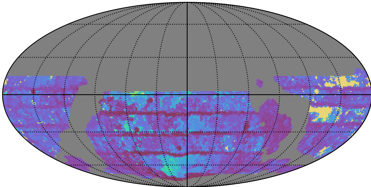
weather_cloudso31v3.4_10yrs WFD z band: Max Inter-Night Gap
