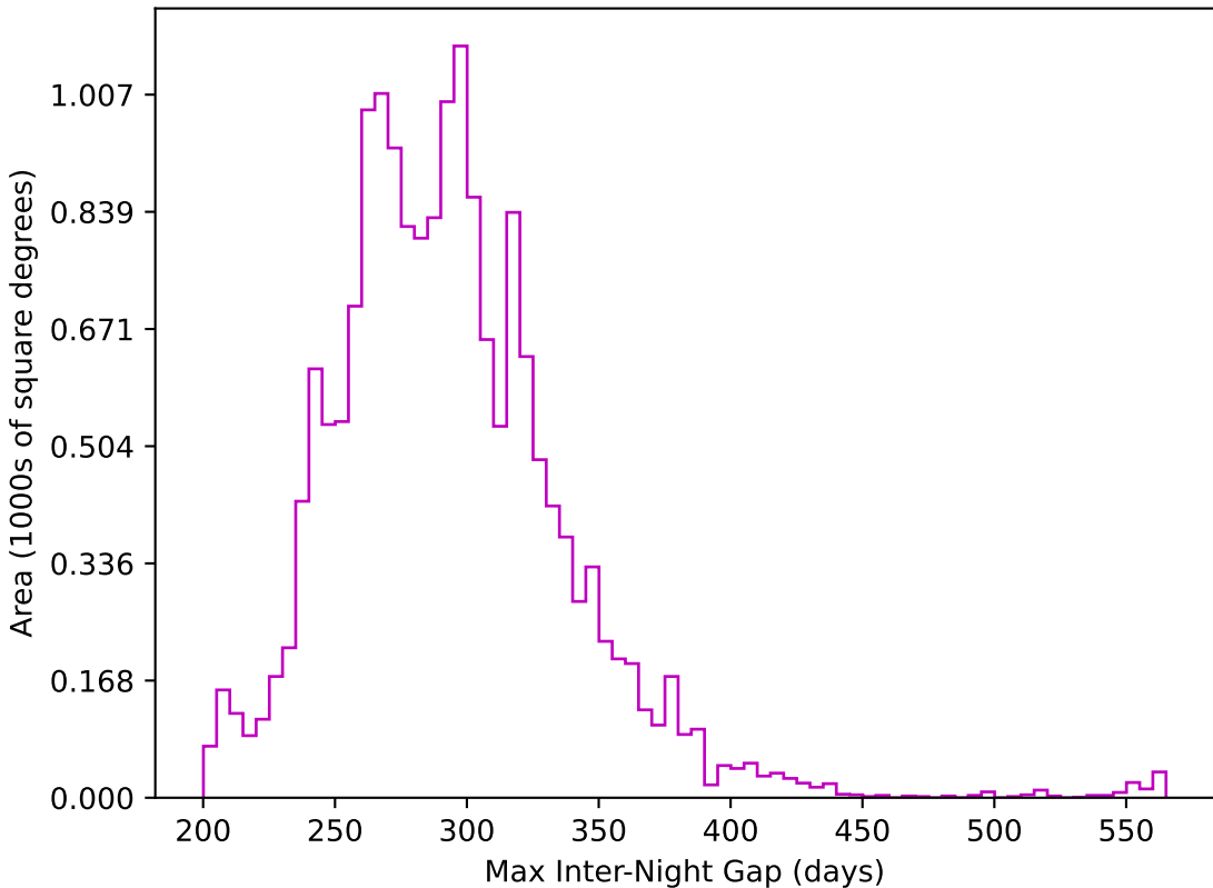
weather_cloudso31v3.4_10yrs WFD z band: Max Inter-Night Gap
