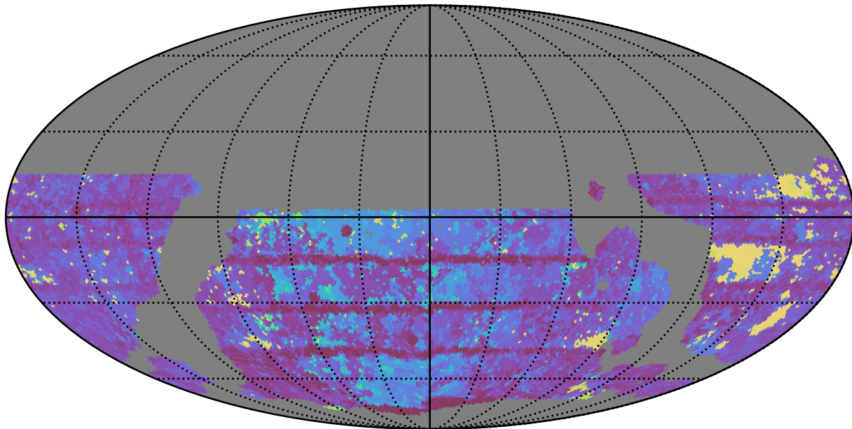
weather_cloudso31v3.4_10yrs WFD y band: Max Inter-Night Gap
