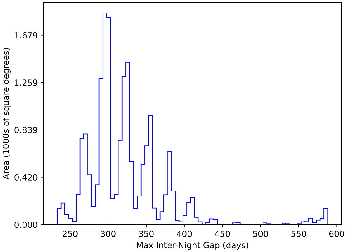
weather_cloudso31v3.4_10yrs WFD y band: Max Inter-Night Gap
