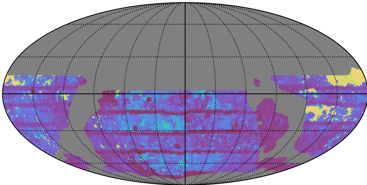
weather_cloudso31v3.4_10yrs WFD r band: Max Inter-Night Gap
